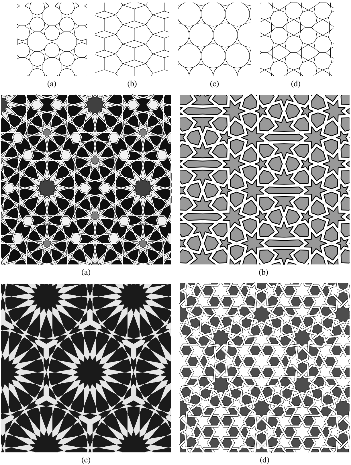
Figure 9 Sample results not found in the literature. The pattern in (a) is similar to one found in Abas and Salman [2, p. 93], using extended rosettes instead of ordinary rosettes. The other three patterns are based on previously unused tilings.
