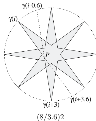
Figure 2 An (n/d)s star for non-integral d .
