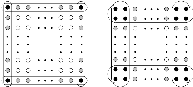
Fig. 2. Approximate C^0 boundary points and C^1 boundary points.
