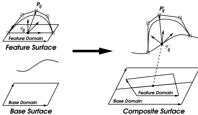
Fig. 1. Surface Pasting.
